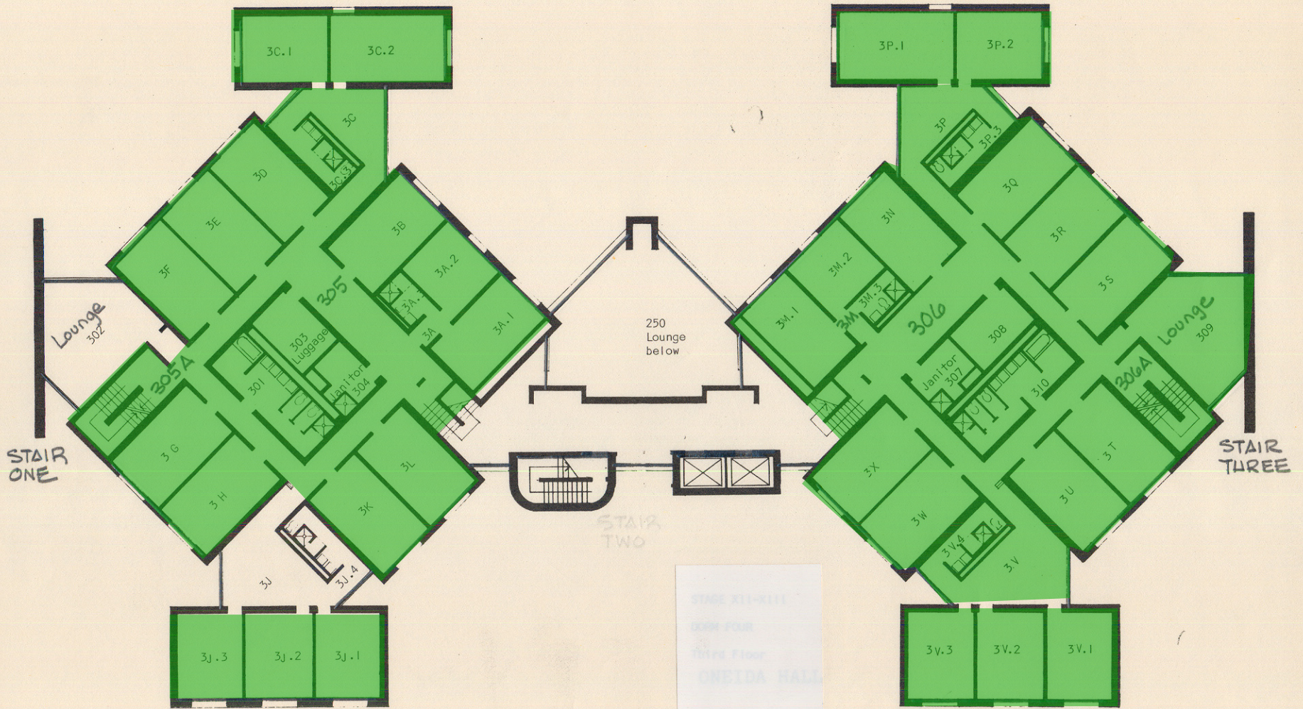
BINGHAMTON UNIVERSITY ONEIDA HALL (COLLEGE IN THE WOODS) THIRD FLOOR PLAN BLDG. NO. 045 NORTH
