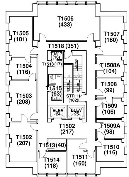
FIFTEENTH FLOOR PLAN Gross Area: 3,822 sf
