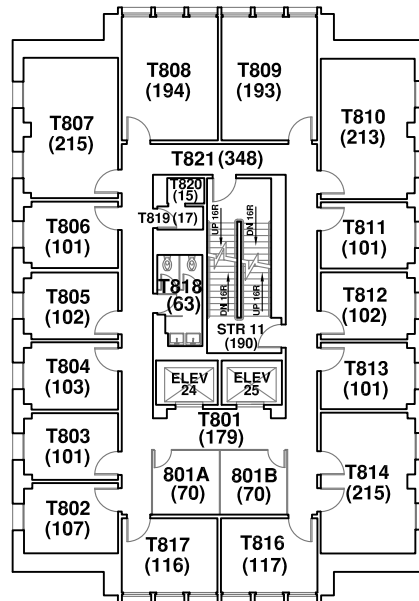
EIGHTH FLOOR PLAN Gross Area: 3,822 sf
