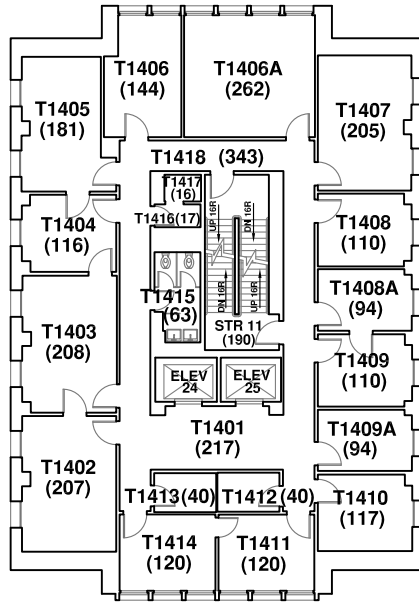
FOURTEENTH FLOOR PLAN Gross Area: 3,822 sf
