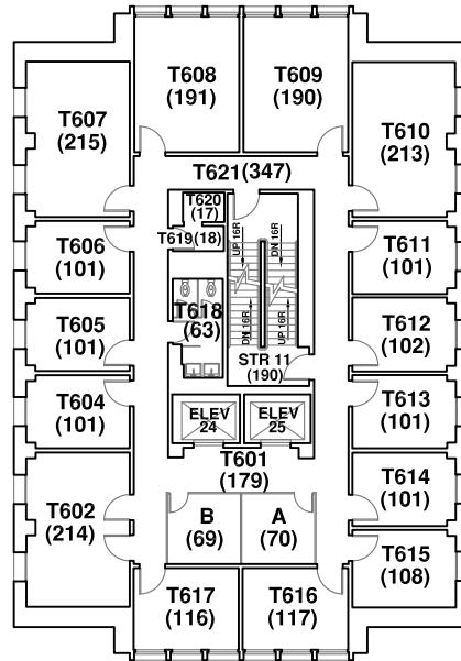
SIXTH FLOOR PLAN Gross Area: 3,822 sf
